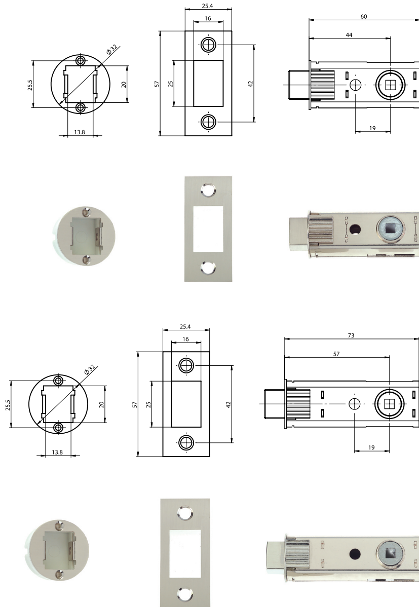
Privacy Bolt
