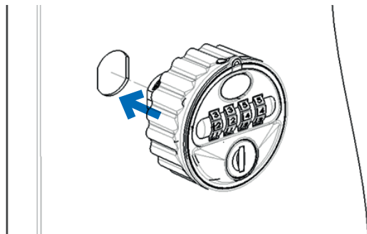
DIAGRAM 1. Position 2800/2810 through door panel as shown.
